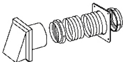
1M Ducting Kit 4" / 100mm Diameter WHT Or BRN Or Tumble Dryer
